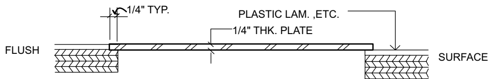
COUNTER CUTOUT FOR OTHER SURFACES
