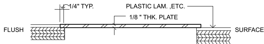
COUNTER CUTOUT FOR OTHER SURFACES
