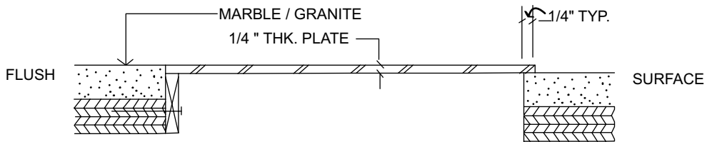
COUNTER CUTOUT FOR MARBLE / GRANITE
